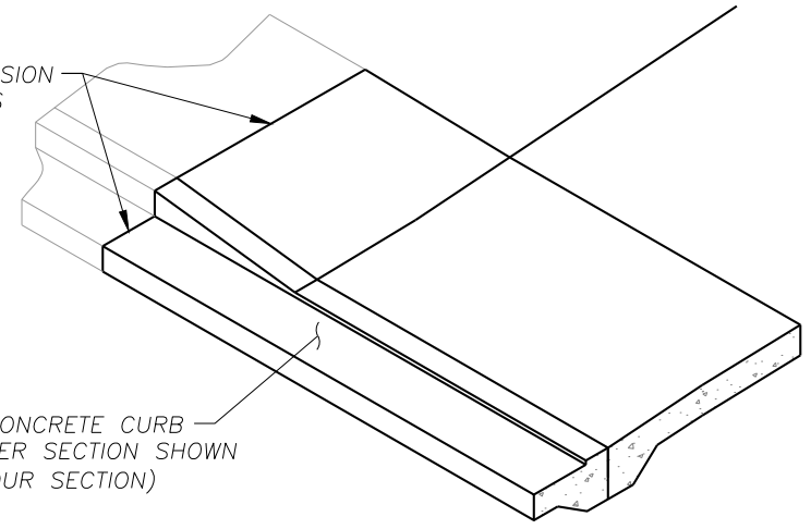
HALF ISOMETRIC
