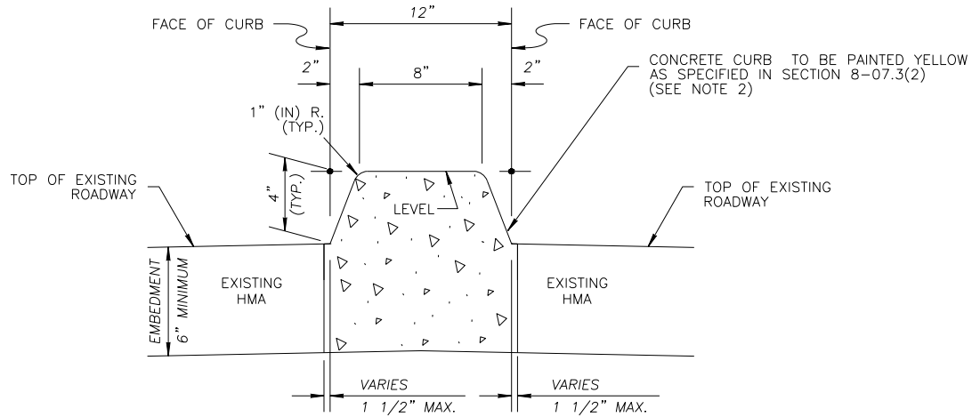
CROSS SECTION DUAL-FACED CEMENT CONC. TRAFFIC CURB TYPE 1 (PREFERED)
