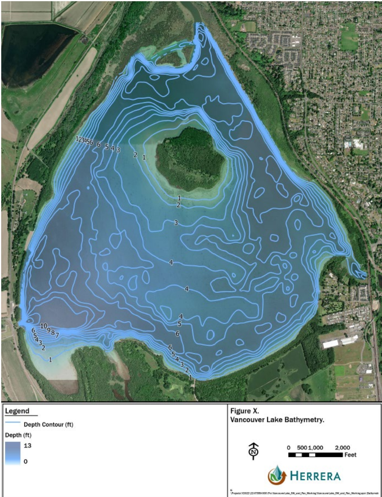
Figure 2. Bathymetry Map of Vancouver Lake (June 15, 2019). Source: USACE (2009)
