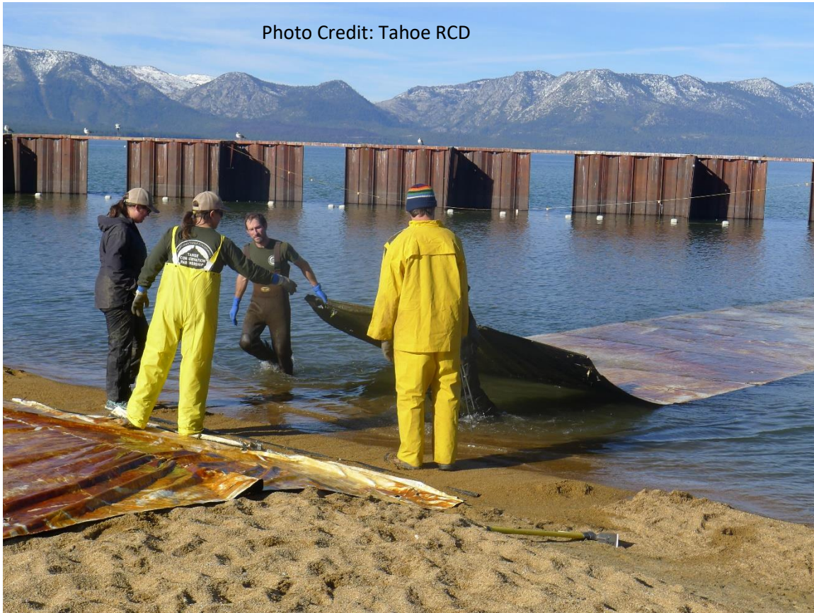
Figure 8. Workers using bottom barriers
