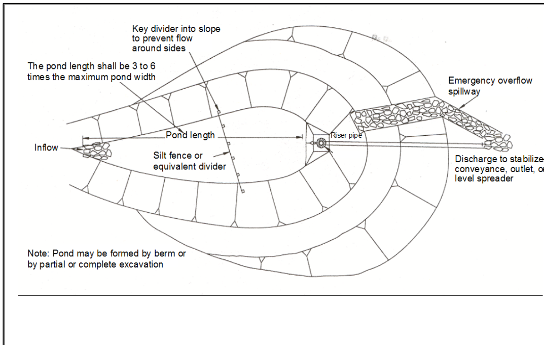
Figure 8.30: Sediment Pond Plan View
