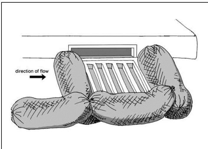
Figure 8.18: Illustration of Storm Drain Inlet Protection
