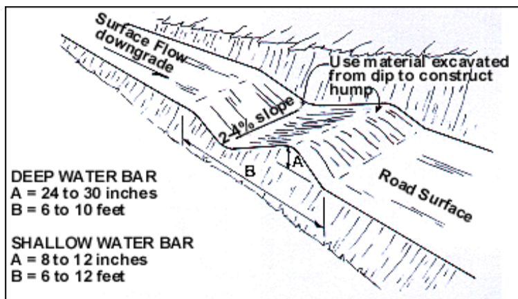
Figure 8.14: Water Bar
