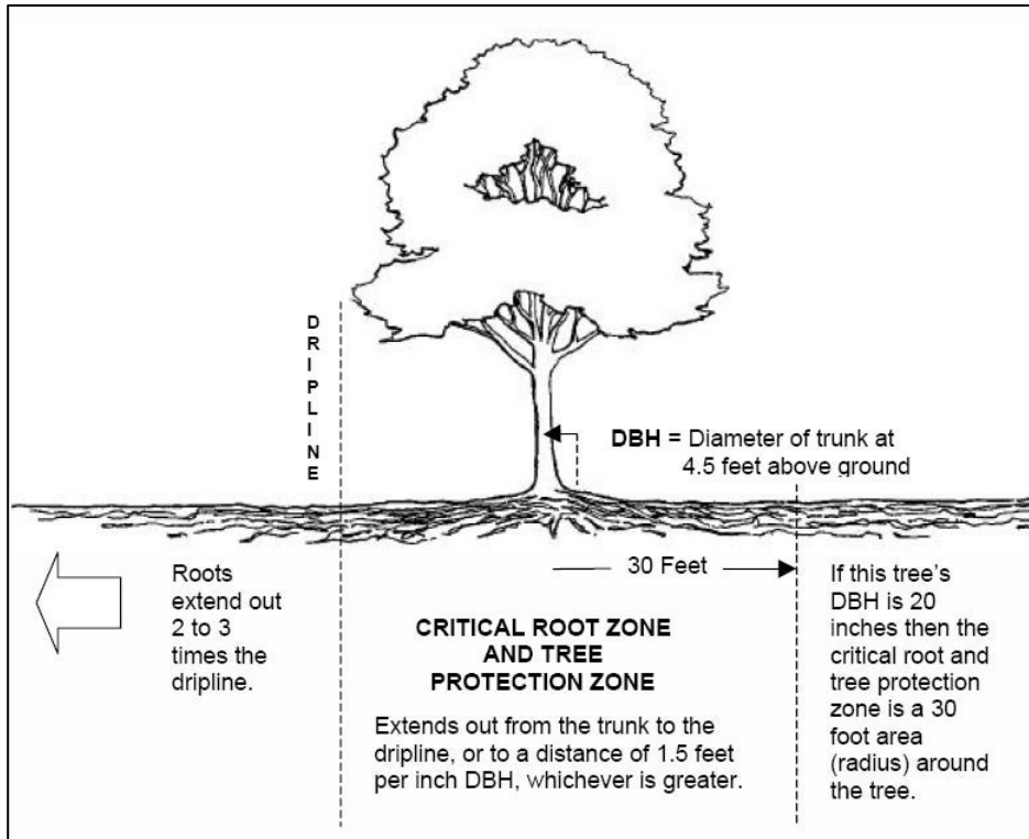
Figure 8.1: Illustration of Tree's Critical Root Zone
