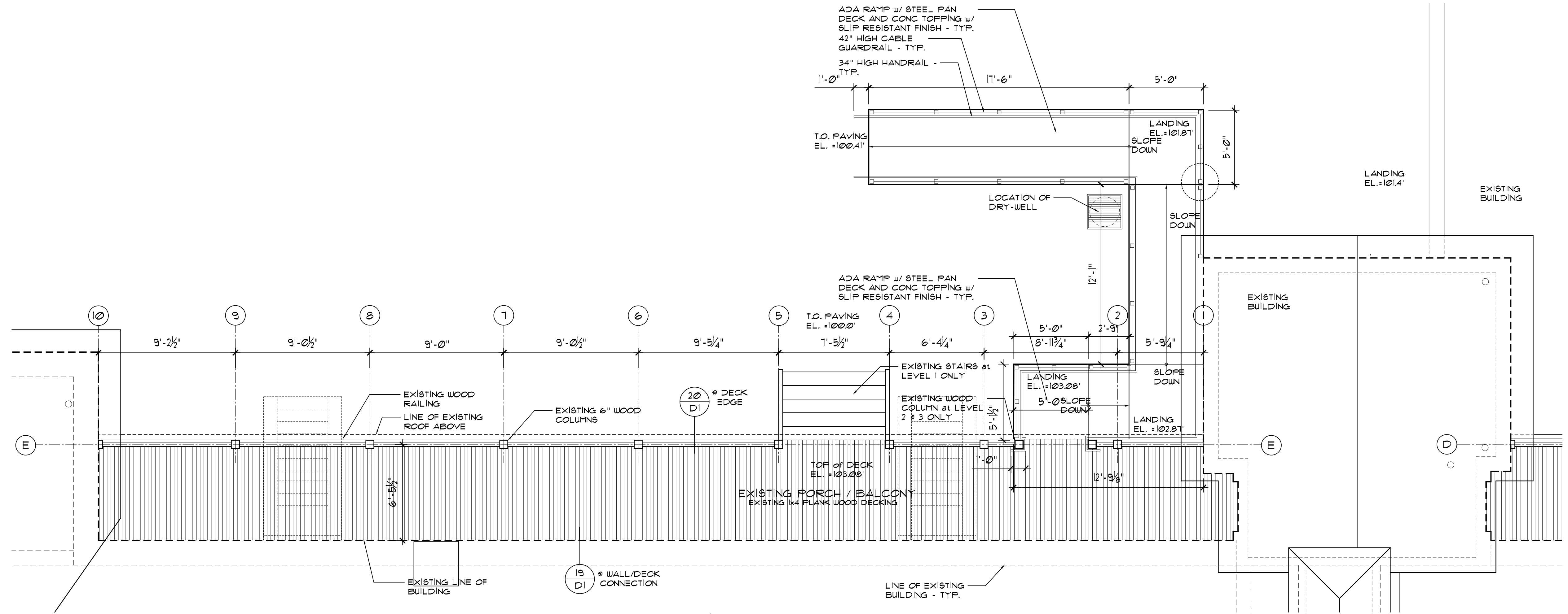
NORTH PORCH / BALCONY PLAN SCALE: 1/4" = 1'-0"
