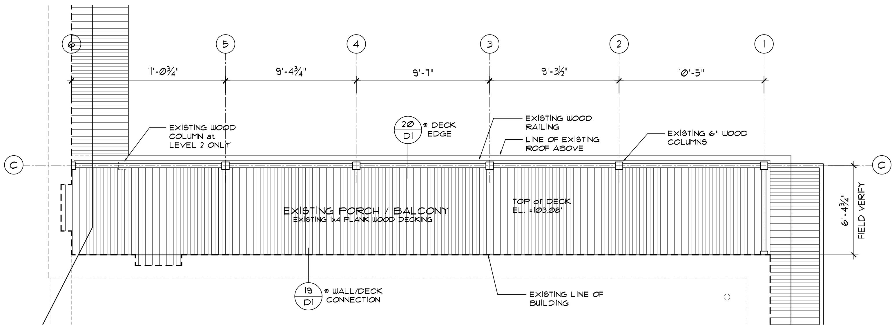
NORTHEAST PORCH / BALCONY PLANS SCALE: 1/4" = 1'-0"
