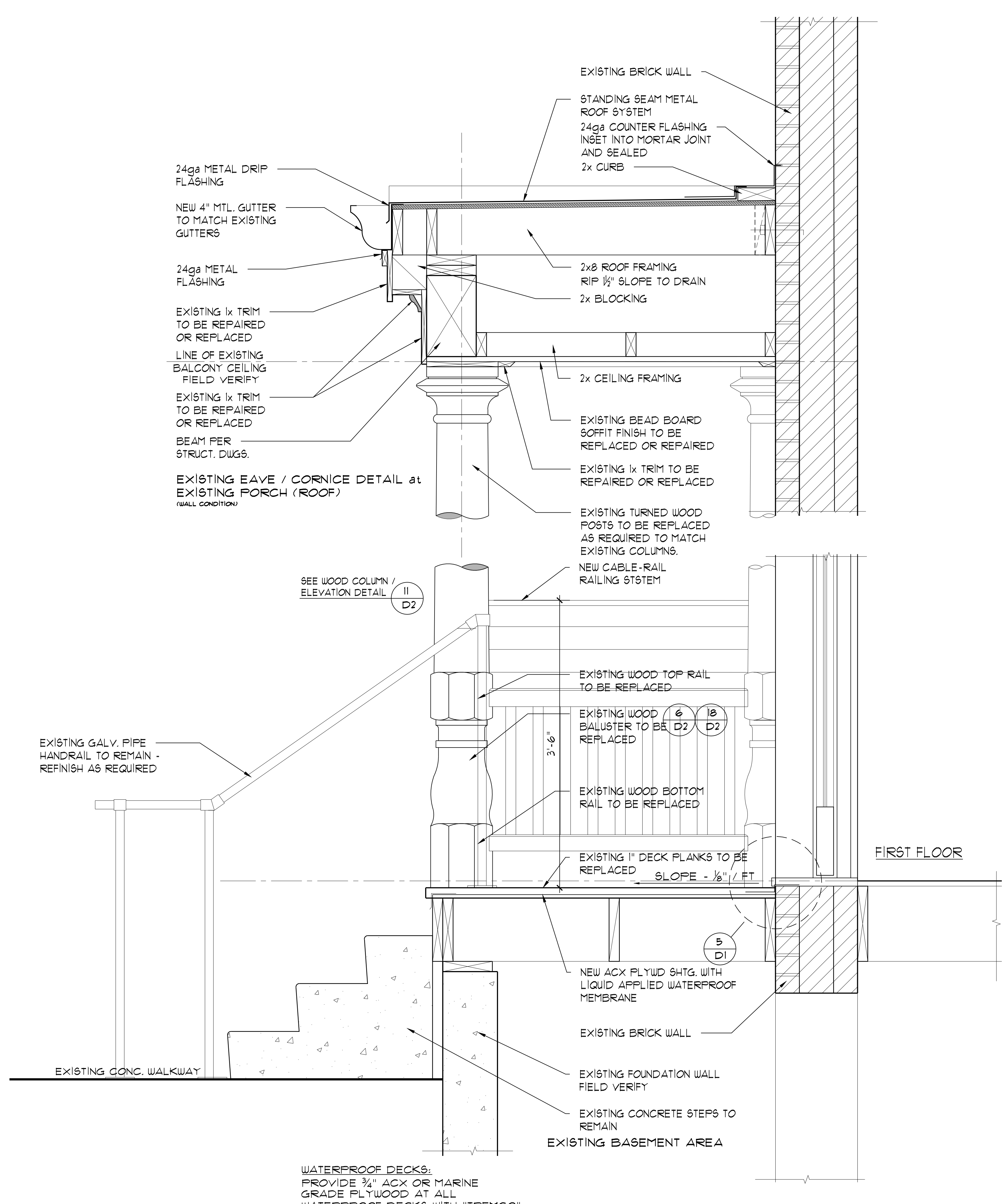
12 ROOF DETAIL @ EAST ENTRY PORCH SCALE: 3" = 1'-0"
