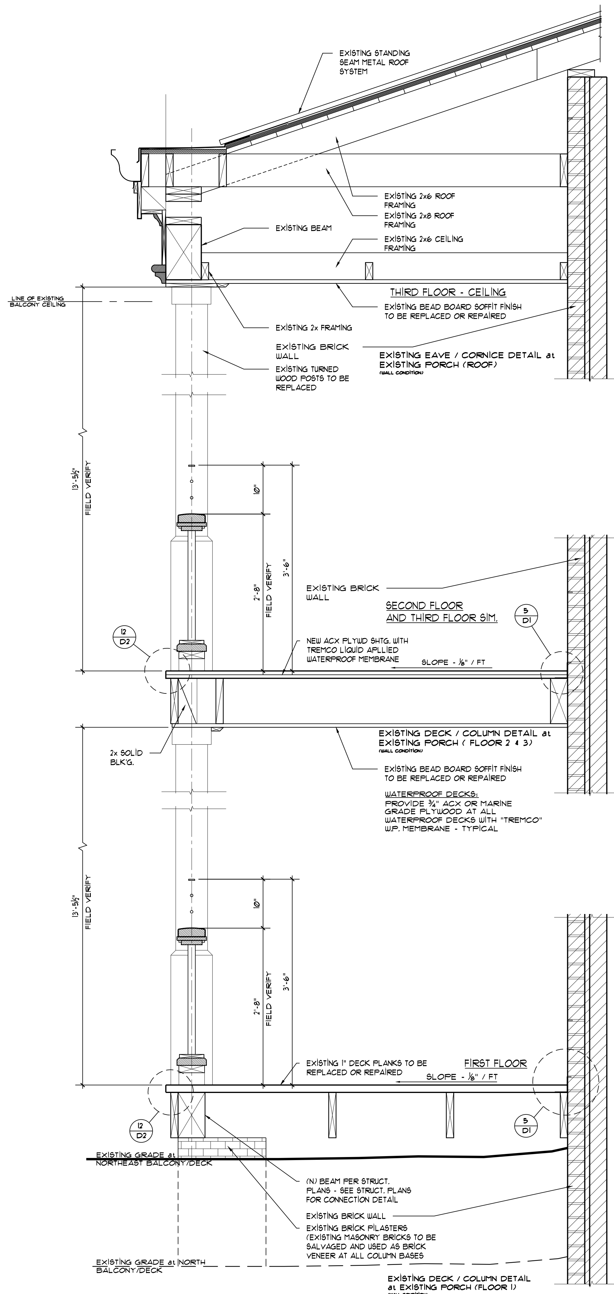
20 PORCH WALL / SECTION DETAIL SCALE: 1" = 1'-0"
