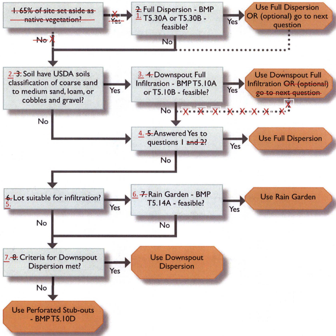
Figure 2: BMP Selection Process for Roofs
