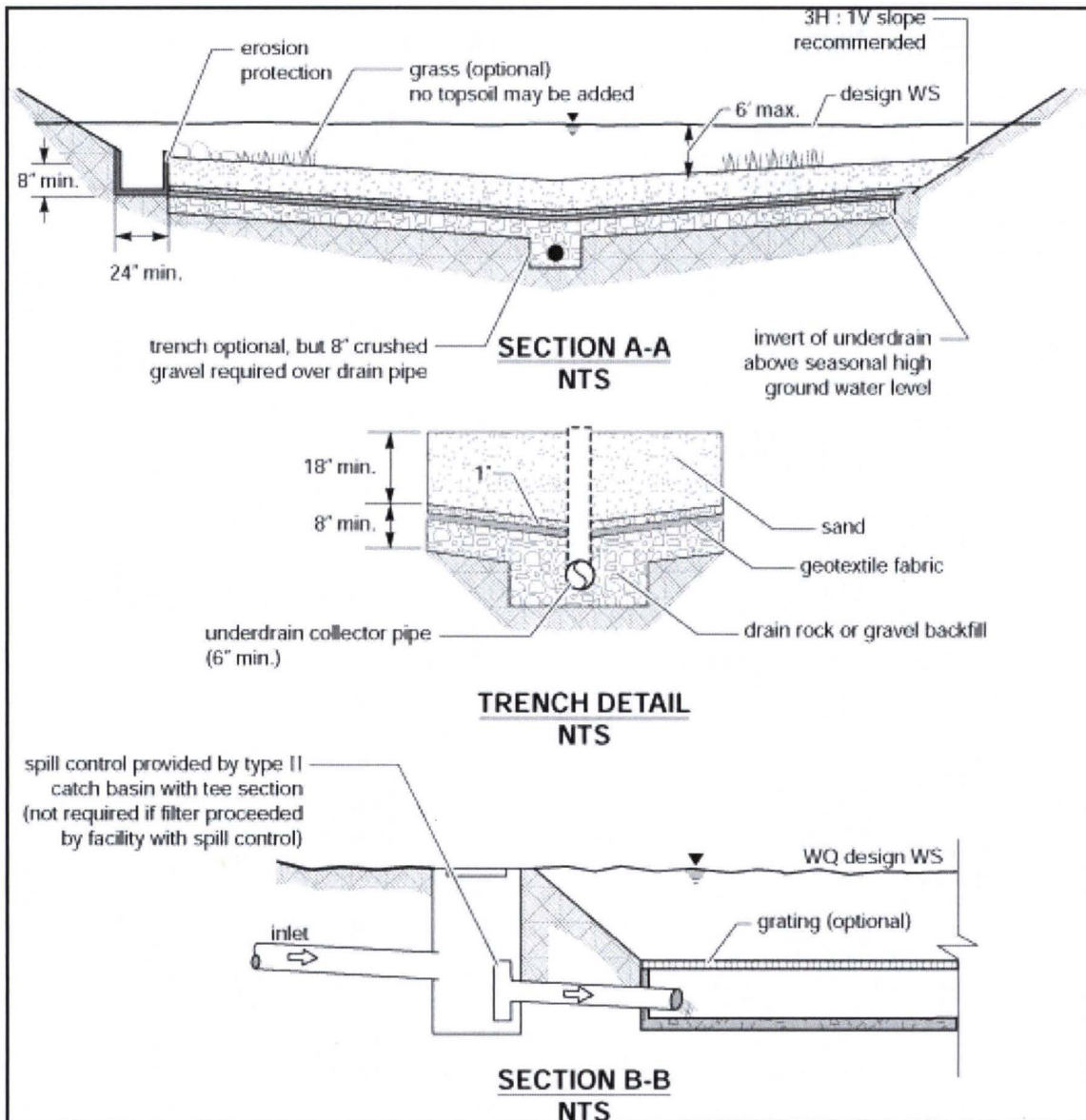
Figure 4.10: Sand Filter with Flow Spreader - Plan Section View
