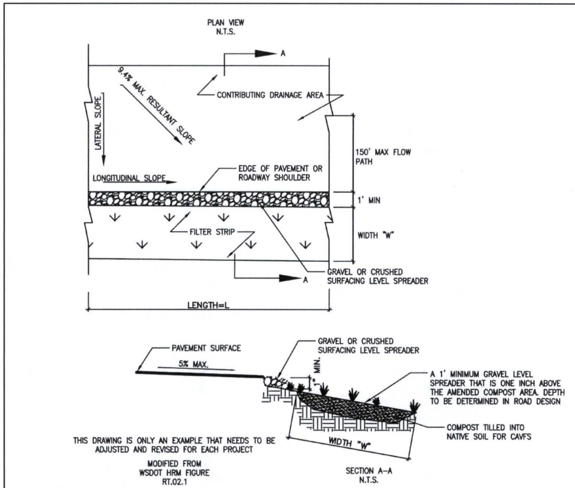
Figure 4.25: Compost Amended Vegetated Filter Strip Typical
