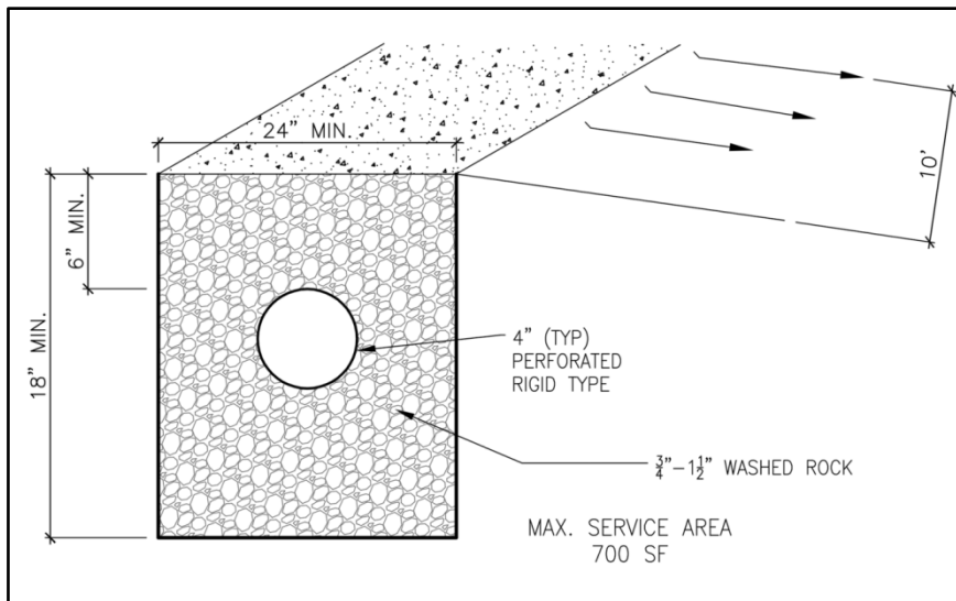
Figure 22: Downspout Dispersion Trench Cross-Section
