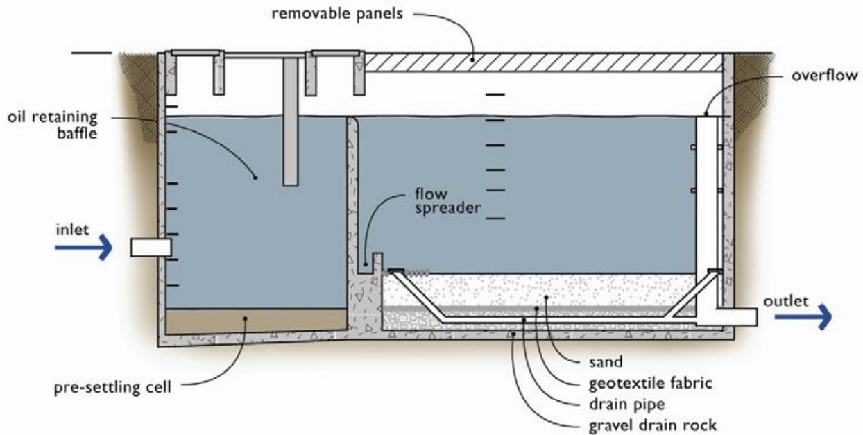
SIDE PROFILE
