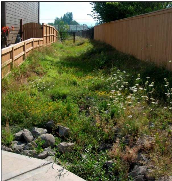
Example Typical Biofiltration Swale
