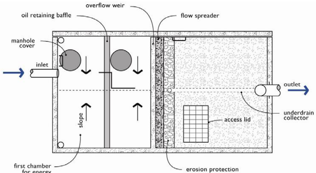
BIRD'S-EYE VIEW
